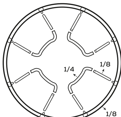
10', 12' Trampoline
